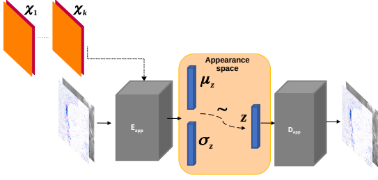
Fig. 4: The Appearance Module pipeline
