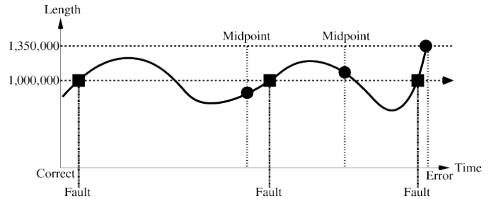
Fig. 4: Reverse Expression Watchpoint.
